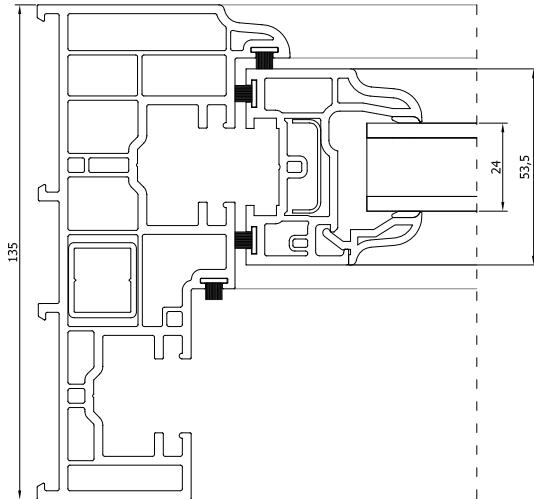
SECTION D (D1 MIRROR)
