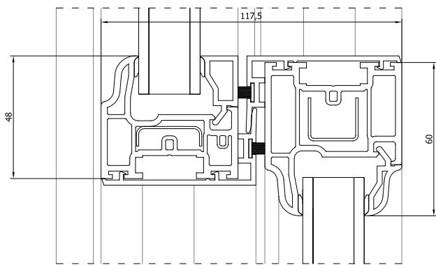
SECTION D (D1 MIRROR)
